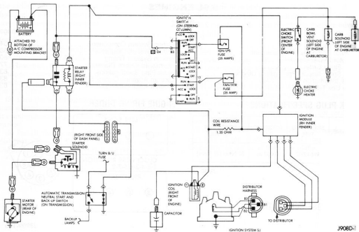
Fig. 1 5.9L Ignition Schematic
